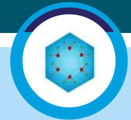
Into smaller Hexagonal clusters
