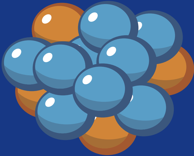
Regular Water Cluster (15-20 Molecules)
