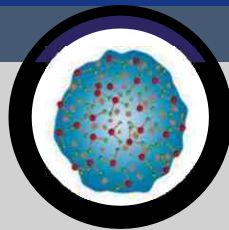
To form water molecule clusters
